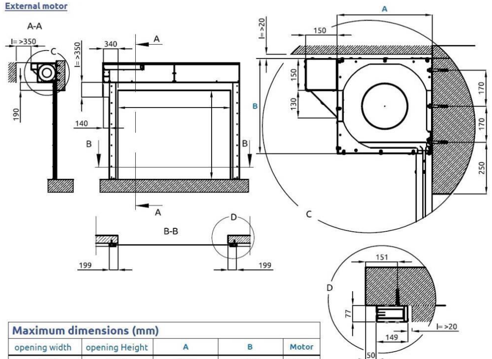
External motor
