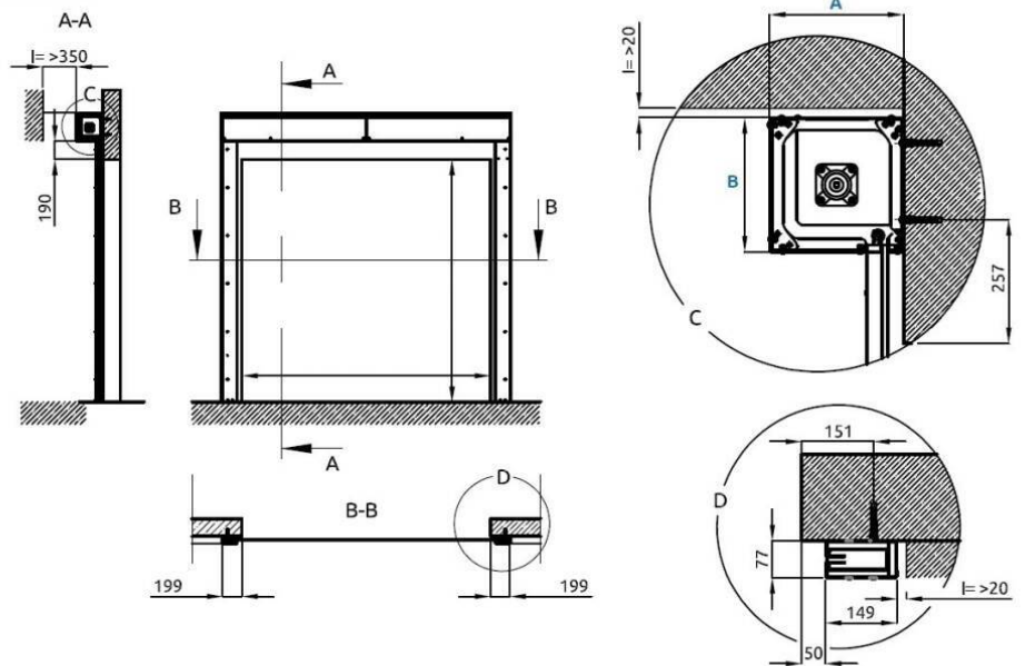
Internal motor
